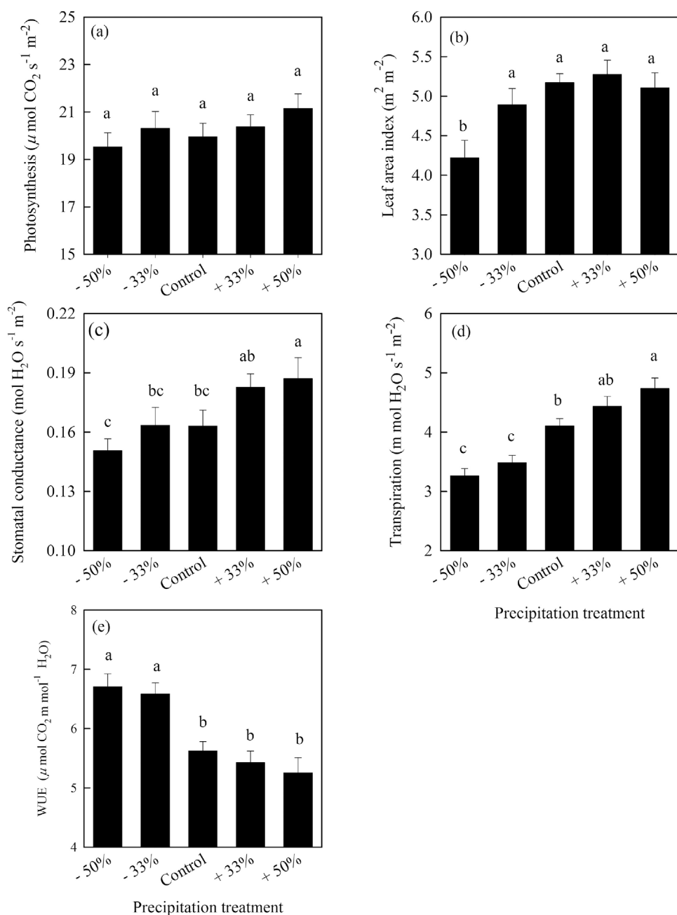
Fig. 4. Mean leaf photosynthesis (a), leaf area index (LAI) (b), stomatal conductance (c), transpiration (d), and water use efficiency (WUE) (e) in each precipitation treatment during the growing seasons. Error bars represent standard errors. Different letters over the bars of litter indicate statistically significant differences among the precipitation treatments.
