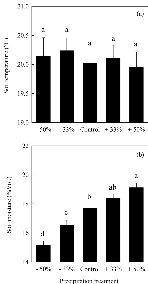
Fig. 2. Mean soil temperature and soil moisture at 10 cm depth in each precipitation treatment during the growing seasons. Error bars represent standard errors. Different letters over the bars of litter indicate statistically significant differences among the precipitation treatments. There was no significant difference in soil temperature among the precipitation treatments.
