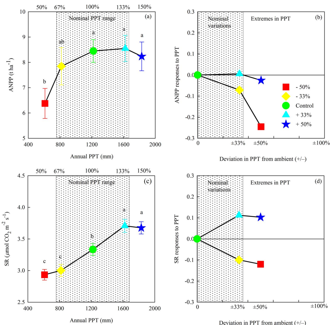
Fig. 3. The relationships between aboveground net primary production (ANPP) and annual precipitation (PPT) or between soil respiration (SR) and PPT across two-year data. (a) ANPP-PPT relationship displayed single negative asymmetry model and (c) SR-PPT relationship displayed an “S” curve model. (b) ANPP-PPT relationship and (d) SR-PPT relationship re-drawn to emphasize the comparative magnitudes in ANPP and SR, respectively. Error bars represent standard errors. Different letters over the bars of litter indicate statistically significant differences among the PPT treatments.
